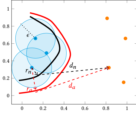
(a) Toy problem demonstrating that adversarial training can result in counterfactuals that are both costlier and further from the desired class manifold. The natural decision boundary is shown in black, the adversarial boundary in red. \epsilon -Adversarial training creates a necessary recourse cost c_a = \epsilon > c_n , and yields a distance in the resulting recourse to the desired manifold of d_a > d_n
