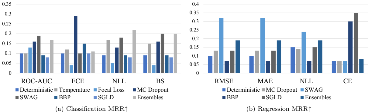
Figure 8: MRR of the UQ methods for each metric, each is macro-averaged from the reciprocal ranks of the results of all corresponding backbone models on all randomly split datasets.
