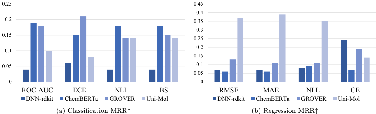
Figure 9: MRR of the UQ methods for each backbone model, each is macro-averaged from the reciprocal ranks of the results of all corresponding UQ methods on all randomly split datasets.
