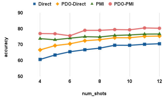
Figure 4: We show the mean accuracy over 5 topic classification datasets across different numbers of in-context training examples (from 4 to 12) under FewShotUP . The backbone LLM is LLaMA-7B. PDO ’s improvement is consistent with different numbers of samples.
