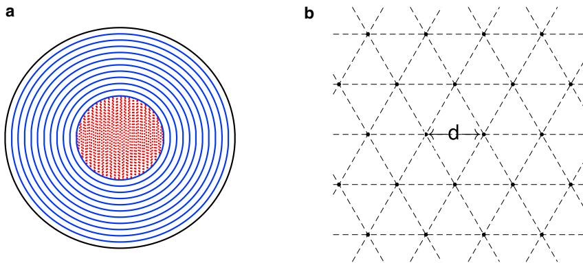
FIGURE 1 Configuration of packed DNA inside a bacteriophage capsid. ( a ) Side view parallel to the axial direction. The black circle represents the protein capsid, and the blue curve describes the ordered structure of the DNA chain. The red dots in the center describe the disordered core region. ( b ) Side view perpendicular to the axial direction; each dot represents the intersection of a DNA segment with the cross section. The dots are locally arranged in a hexagonal lattice structure. Note that the distance between neighboring DNA segments may change in space as a function of the distance to the center of the capsid. To see this figure in color, go online.
