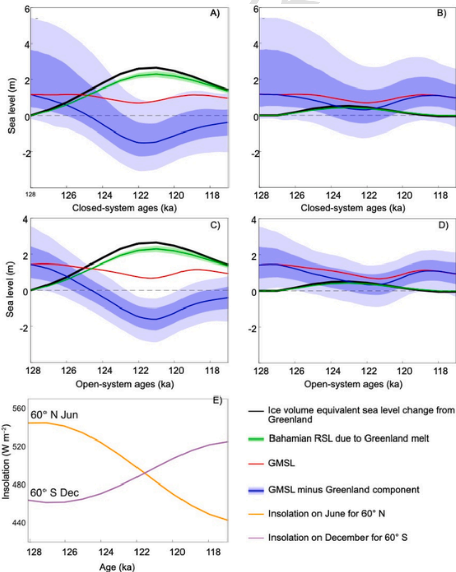
Fig. 8. Ice volume equivalent sea-level change for GrIS melt using two melt scenarios from Calov et al. (2015), black curves. A and B show results using closed-system ages; C and D using open-system ages for the median GMSL (red line). Resulting relative sea-level change in The Bahamas (green curve, mean and 1 standard deviation). Note that we omit uncertainties here for clarity; uncertainty bands can be seen in Fig. 6A. The non-Greenland component that drives sea-level change in The Bahamas is in blue (solid line is median, shading is 68% and 95% percentile envelope). E) Summer insolation curves for northern and southern hemispheres (Berger and Loutre, 1991).
