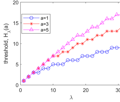
Figure 2: Threshold H_\lambda(a) versus \lambda for the per-UE stochastic arrival problem at different a . p_s = 0.5 , p_g = 0.5 .
