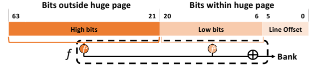
Figure 16: Bank address hash function in a huge page. The higher bits outside of the huge page are hashed and then xored with the hash of bits within the huge page to generate the bank address.
