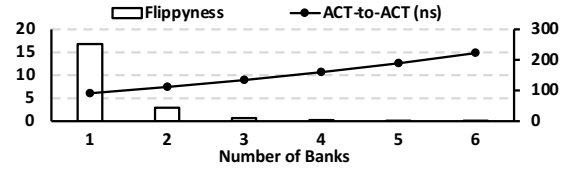
Figure 7: Results from Figure 6 divided by the number of banks and hammering iterations (flippiness) and the average time between two ACTs per bank (ACT-to-ACT).
