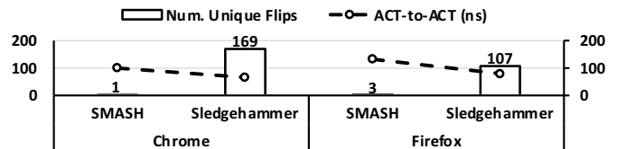
Figure 23: Number of flips per hour and average ACT-to-ACT.
