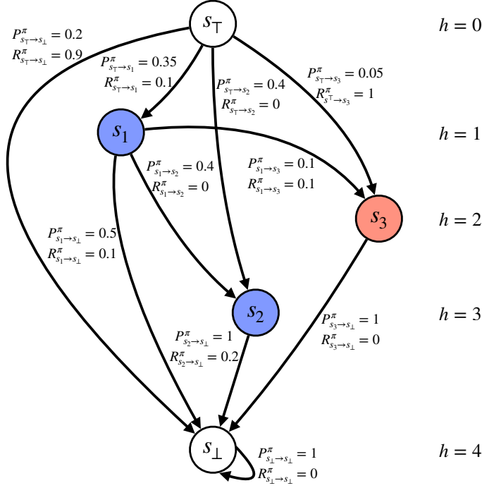
Figure 2: Illustration of an MRP \mathfrak{M}_{\mathcal{S}^{\text{rch}}}^{\pi} with \mathcal{S}_{\pi} = \{s_1, s_2, s_3\} and \mathcal{S}^{\text{rch}} = \{s_1, s_2\} . In the original MDP M , s_1 \in \mathcal{S}_1 , s_2 \in \mathcal{S}_3 , and s_3 \in \mathcal{S}_2 . The edges are labeled with the values of P_{s \rightarrow s'}^{\pi} and R_{s \rightarrow s'}^{\pi} . Notice that (1) there are no edges from s_2 \rightarrow s_3 or s_3 \rightarrow s_2 because trajectories cannot go from later layers to earlier ones; (2) since s_3 \notin \mathcal{S}^{\text{rch}} , there is no edge from s_3 \rightarrow s_2 , and instead we have P_{s_3 \rightarrow s_{\perp}}^{\pi} = 1 and R_{s_3 \rightarrow s_{\perp}}^{\pi} = 0 ; (3) s_{\perp} is an absorbing state with no rewards.
