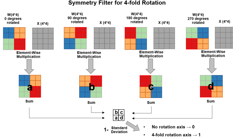
Figure 2: Graphic demonstration of custom symmetry filter for 4-fold rotation. A custom 4-fold rotation filter is defined by rotating a randomly defined matrix four times for four different kernels. Then, we perform the element-wise multiplication on the four kernels with the gray region, a sliding window from the symmetry image. The sum of the matrix is calculated as a, b, c, and d for four output matrices. Using one minus the standard deviation of the a, b, c, and d, the indicating feature value is extracted to determine the existence of a 4-fold rotation in the center of the sliding window.
