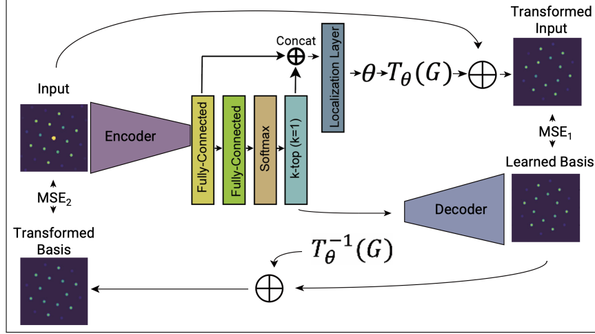
Figure 1: Schematic drawing of cycle-consistent spatial transforming autoencoder.
