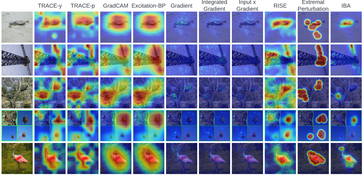
Figure 7. Visualizations of TRACE and popular attribution methods on images from ILSVRC2012.
