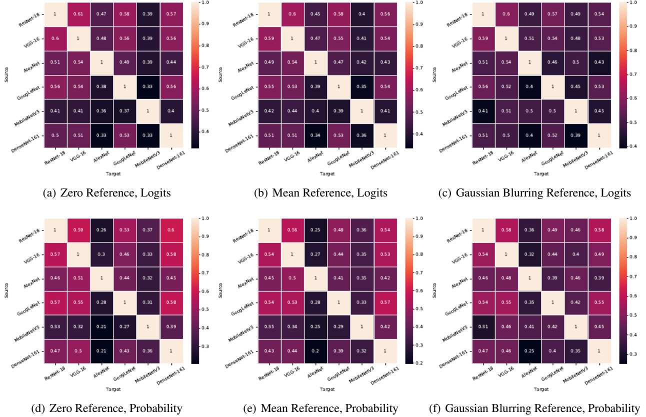
Figure 16. The transferability of the trajectory among 6 different DNNs. In each subfigure, the y -axis is the list of source models, which the trajectories are optimized over. The trajectories are then tested over the target models listed on the x -axis. The upper row is the result when the predicted logits are used as the measurement. The lower row is the result of the predicted probability. And each column represents a certain type of reference value. Results show that AlexNet and MobileNetV3's best trajectories are the most distant from others.
