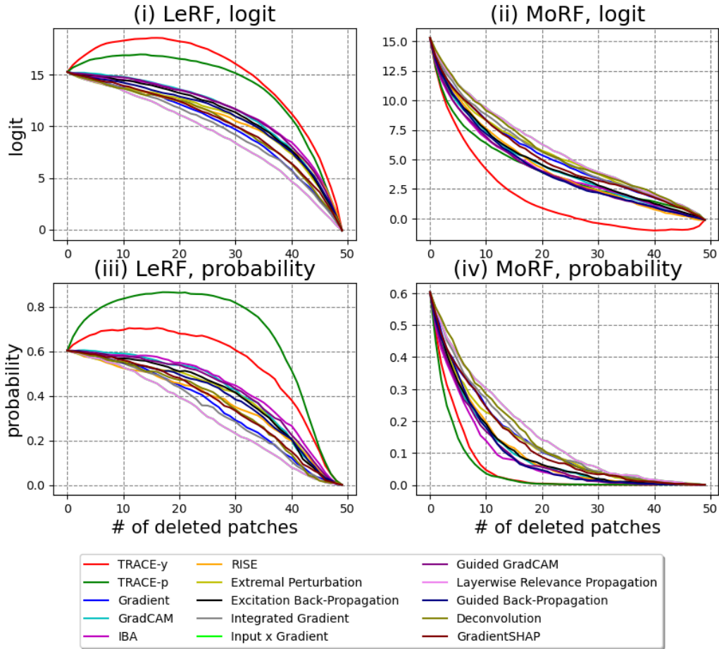
Figure 11. The comparison between the deletion tests of TRACE and more attribution methods
