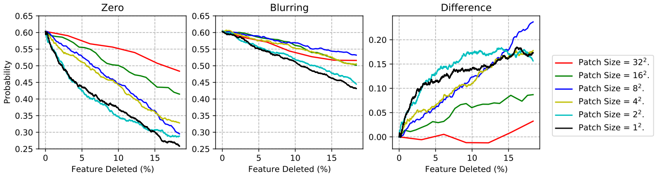
Figure 4. Random deletion tests with (a) zero (b) blurring reference; and (c) difference between (a)(b). 6 different patch sizes are tested.
