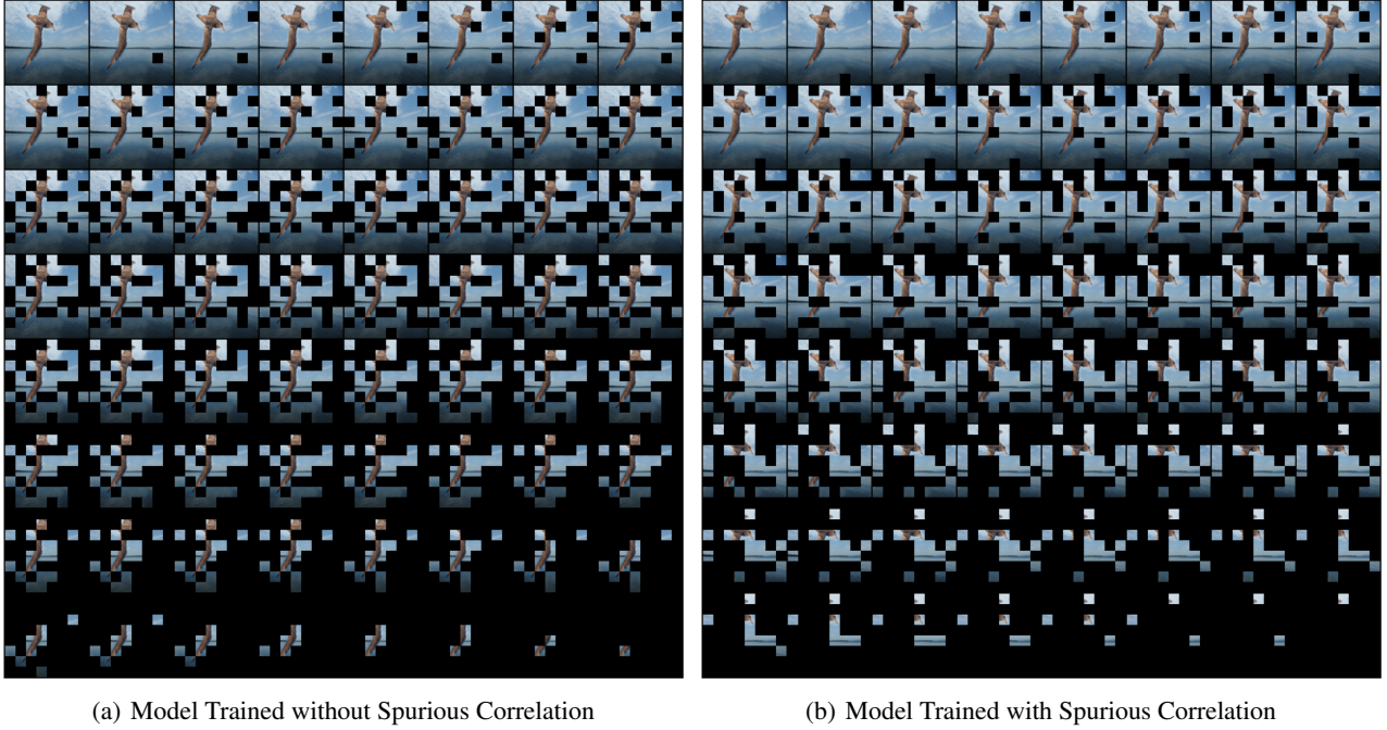
Figure 15. The demonstration of the LeRF deletion process of TRACE-Le-Mo on a testing image of the waterbird dataset. The label is associated with the object (bird). In (a), the model is trained on the non-spurious training set, where the ratio of the group sizes is (waterbird, water):(waterbird, land):(landbird, water):(landbird, land) = 1 : 1 : 1 : 1. On the contrary, in (b), the model is trained on the spurious correlated training set, where the ratio among the four groups is 999 : 1 : 1 : 999. This suggests that model (b) may rely on the background to make the prediction instead of the object. Since the testing sample is waterbird + water, both models achieve correct predictions with confidence > 1 - 10^{-4} . However, as illustrated in the bottom row of the two deletion processes, the non-spuriously trained model (a) highlights birds' wings, while the spuriously trained model (b) highlights the coastline of the water background. This demonstrates the power of TRACE in detecting the spurious correlated features due to the direct connection between TRACE and model predictions.
