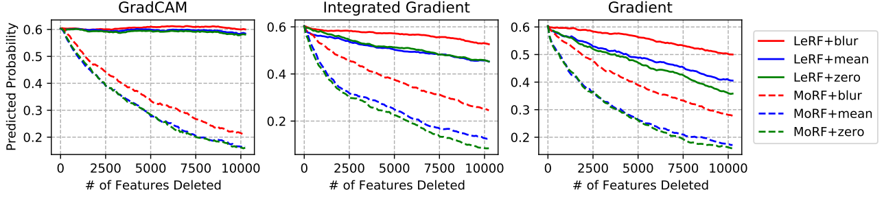
Figure 1. The deletion tests of GradCAM, Integrated Gradient, and Gradient. Solid and dashed curves distinguish between LeRF and MoRF criteria. Different colors represent different reference types. We include the zero, mean, and blurring references.
