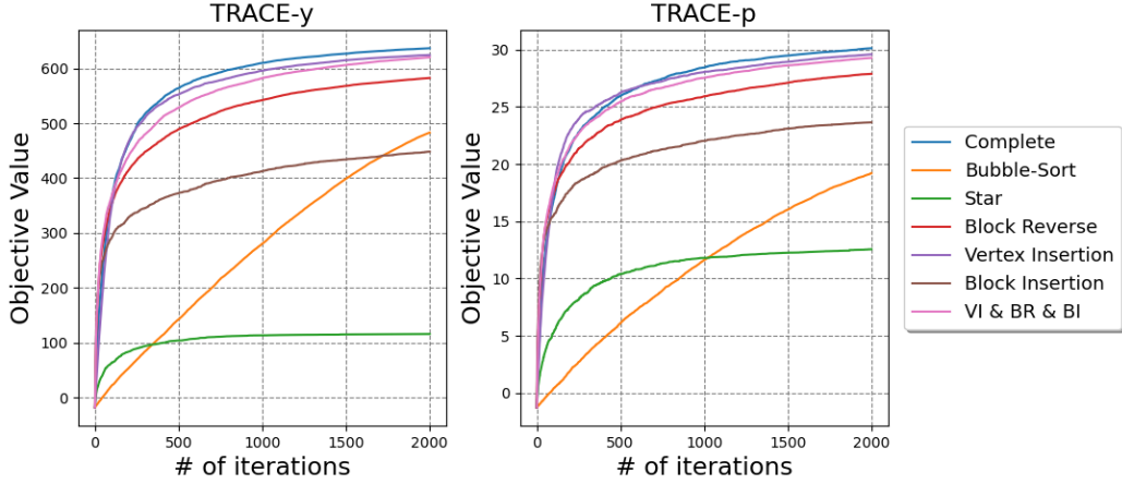
Figure 5. The comparison of different neighbor sets.
