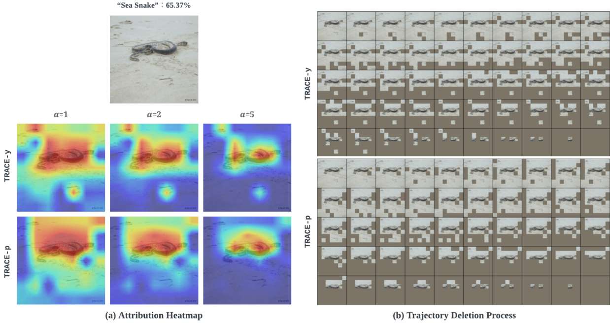
Figure 6. Visualizations of the optimized results of TRACE-y and TRACE-p on the “sea snake” image of ILSVRC2012 validation set. (a) The converted heatmaps \psi with different smoothing factor \alpha . (b) The deletion process is based on the trajectory \tau .
