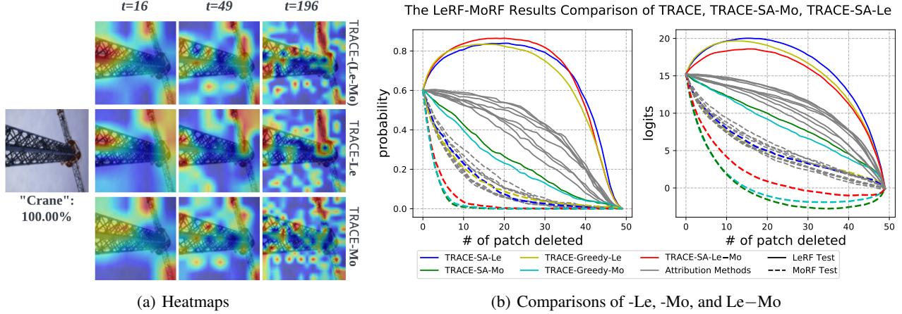
Figure 3. (a) The illustration of the converted heatmaps of the image of a “crane” from the validation set of ILSVRC2012. A ResNet-18 predicts it correctly with the confidence \approx 100.00\% . The smoothing factor \alpha = 2 . Results of TRACE-SA-Le-Mo (top), TRACE-SA-Le (middle), and TRACE-SA-Mo (bottom) are presented. They are implemented w.r.t. the probability. We set t = 4 \times 4 (left), t = 7 \times 7 (middle) and t = 14 \times 14 (right). Here t is the number of square patches of pixels for one image. (b) The comparison of the TRACE-SA-Le-Mo (red), TRACE-SA-Le (blue) and TRACE-SA-Mo (green), TRACE-Greedy-Le (yellow) and TRACE-Greedy-Mo (cyan) under the LeRF (solid) and MoRF (dashed) tests. All explanation methods are also included but plotted indistinguishably just for reference.
