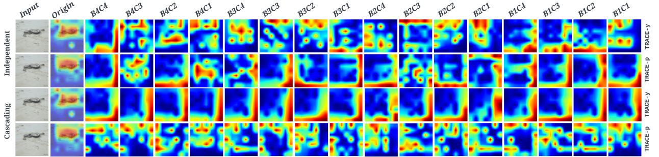
Figure 8. Sanity check using cascading randomization for TRACE. Convolutional layers of pre-trained ResNet-18 are randomized in the independent (upper) and cascading (lower) manners. In the independent randomization, other layers are kept at the pre-trained values. And in the cascading randomization, layers are progressively randomized from left to right (top-down). Here “BaCb” means the b -th convolutional layer in the a -th block.
