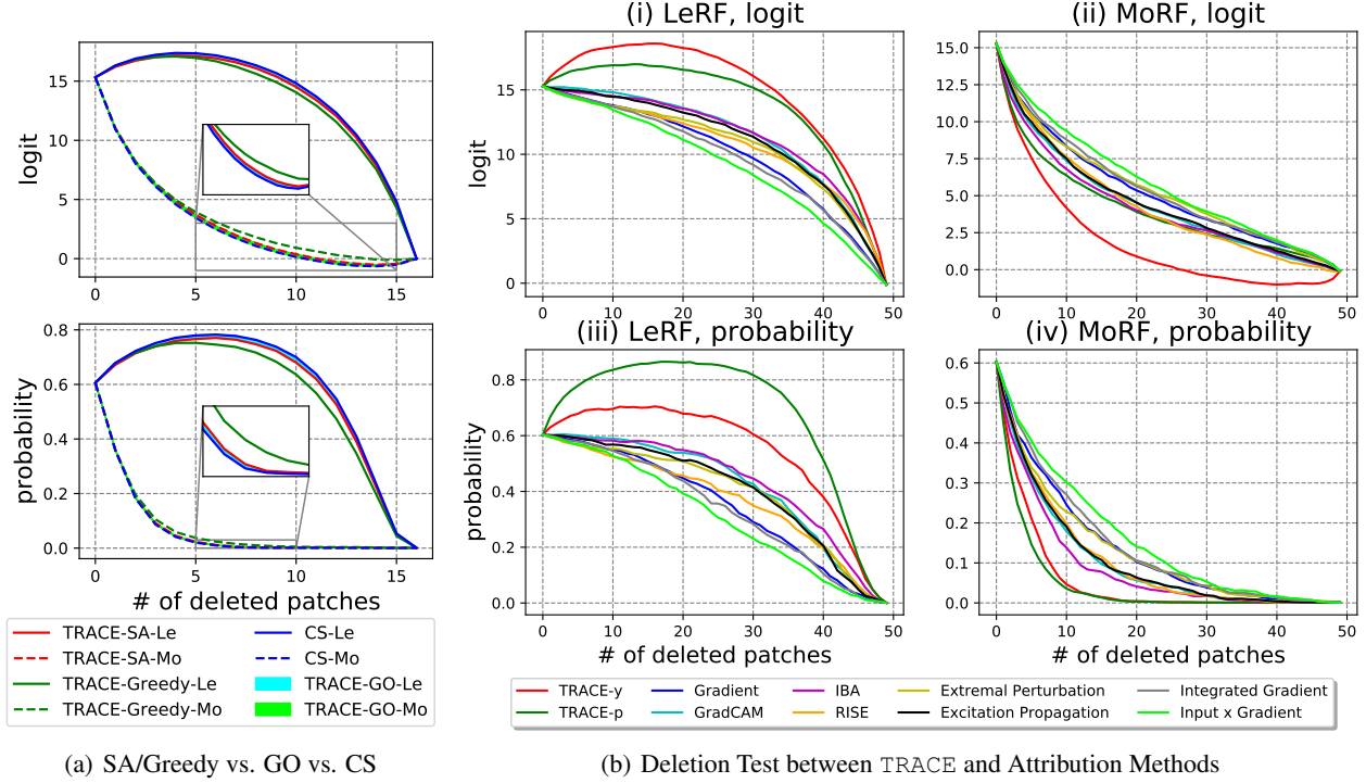
Figure 2. (a) The comparison between TRACE-SA/Greedy, TRACE-GO and Complete Search (CS). CS-Mo/CS-Le are the lower/upper bounds of TRACE-Mo/TRACE-Le, respectively. The blue, red, and green curves are the results of CS, TRACE-SA and TRACE-Greedy. Solid and dashed curves are -Le and -Mo. The optimum TRACE-GO-Le and TRACE-GO-Mo lie in the cyan and lime color areas, respectively, which are notably marginal. (b) Deletion results of the first 200 images from the validation set of ILSVRC2012. In (i)(iii), patches are deleted following LeRF, and in (ii)(iv), patches are deleted following MoRF. The y -axis of (i)(ii) is the output logits of the network, and the y -axis of (iii)(iv) is the predicted probability. x -axis is the number of deleted patches.
