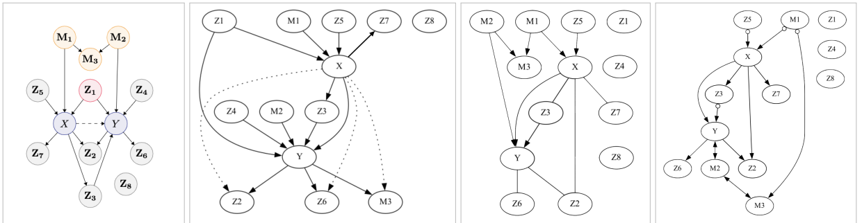
Figure A.2: A ground truth DAG with M-structure versus the DAGs inferred by LDP, PC [ Spirites et al., 2000 ], and FCI [ Spirites et al., 2000 ] (left to right). Causal mechanisms were linear and noise was Bernoulli ( n = 5k ; chi-square independence tests). Only LDP partitioned the variables correctly and returned a valid adjustment set (VAS). LDP returned a VAS at n = 1k , FCI at n = 10k , and PC at n > 10k . Note that LDP does not infer the relations between members of \mathbf{Z} , hence only the paths to X and Y are visualized (abstracted as length-1). Dotted edges indicate that LDP could not distinguish Z_2 from Z_6 , which is expected behavior on this structure. Variables M_1 \in \mathbf{Z}_5 , M_2 \in \mathbf{Z}_4 , and M_3 \in \mathbf{Z}_2 . Experiments use the PC implementation from [ Kalisch and Buhlmann, 2007 ] and the FCI implementation from causal-learn .
