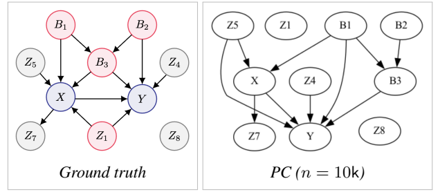
Figure 1: For sample sizes n \leq 10k , classic constraint-based algorithm PC fails to causally partition the data with respect to \{X, Y\} (e.g., by misidentifying confounder Z_1 and instrument Z_5 ). Data generating process is linear-Gaussian (Fisher-z tests; \alpha = 0.005 ). See Figure A.1 for details.
