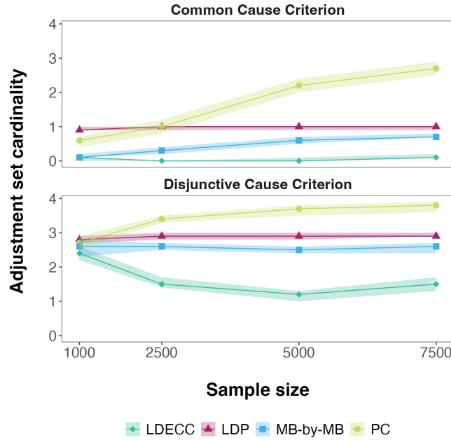
Figure G.3: Adjustment set cardinality for the linear-Gaussian DAG described in Figure 6. The true adjustment set cardinality is one under the common cause criterion and three under the disjunctive cause criterion.
