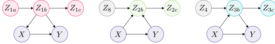
Figure B.3: Example proxy variables for Z_1 , Z_2 , and Z_3 . All Z_{*a} and Z_{*c} are proxies for the corresponding Z_{*b} .
