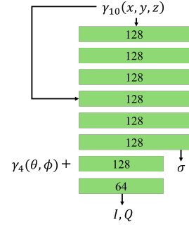
Figure 11. NeWRF’s MLP Architecture. Both Coarse and Fine model use the same architecture.
