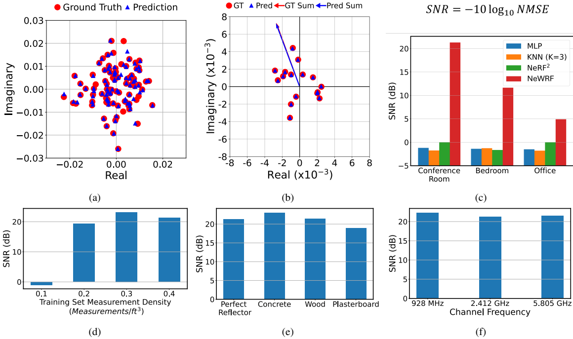
Figure 8. Channel Prediction Results: a) Prediction results for conference room environment. Each dot represents the channel at one test location. b) Predicted channel components (paths) for a single location. Each dot represents a single propagation path. The arrow exhibits the sum of all paths; c) The channel prediction accuracy in different environments compared with baseline methods. d), e), and f) channel prediction accuracy for different training set sample densities, environment materials, and signal frequencies.
