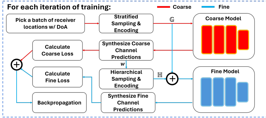
Figure 10. NeWRF’s Training Pipeline
