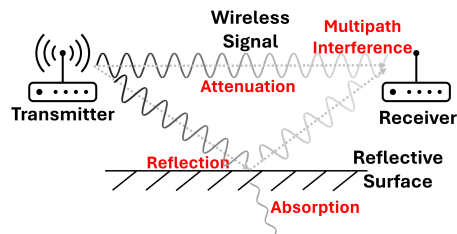
Figure 2. Wireless communication model: Wireless signals emitted by the transmitter experience attenuation, reflection, absorption, multipath interference, etc. before reaching the receiver. Our framework models all of these factors.
