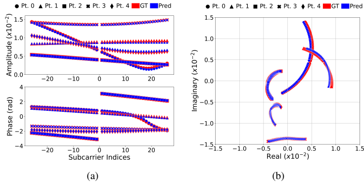
Figure 13. Subcarrier Channel Prediction
