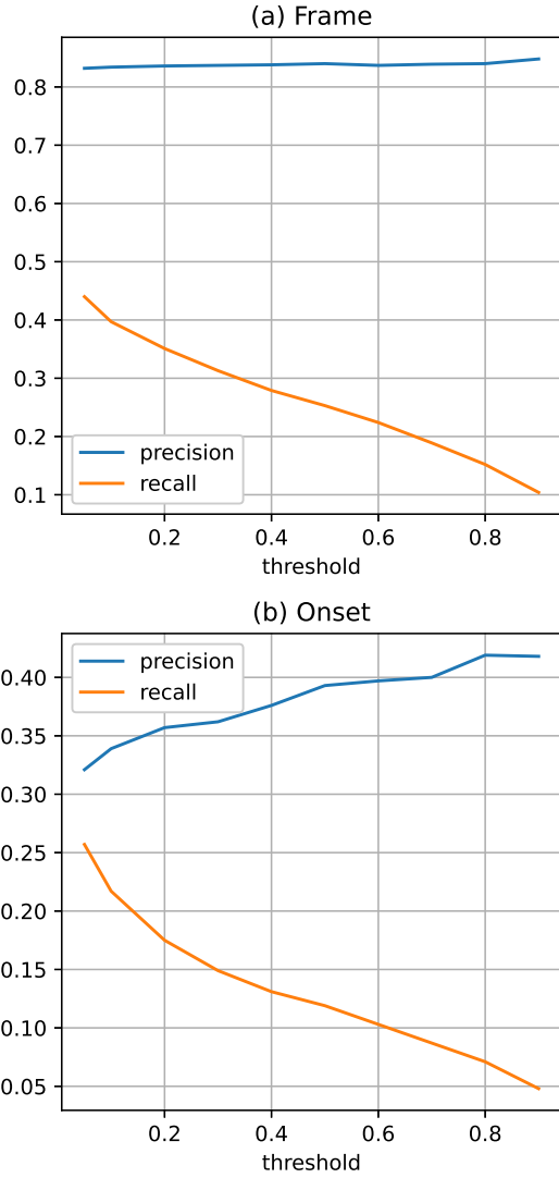
Figure 3. The precision/recall v.s. threshold curves of frame-level and note-level (onset) transcription from Onsets and Frames.
