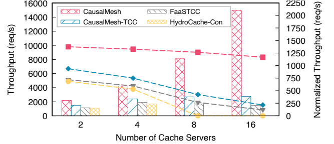
Figure 15: The histogram with y-axis on the left depicts the throughput as we vary the number of servers. The line plot with y-axis on the right shows the normalized throughput by dividing the throughput by the number of servers.
