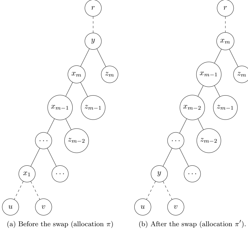
Figure 5: Cyclic swap to show the local median property holds (Lemma 4.10). Solid edges are guaranteed to exist. Dashed edges may or may not exist.
