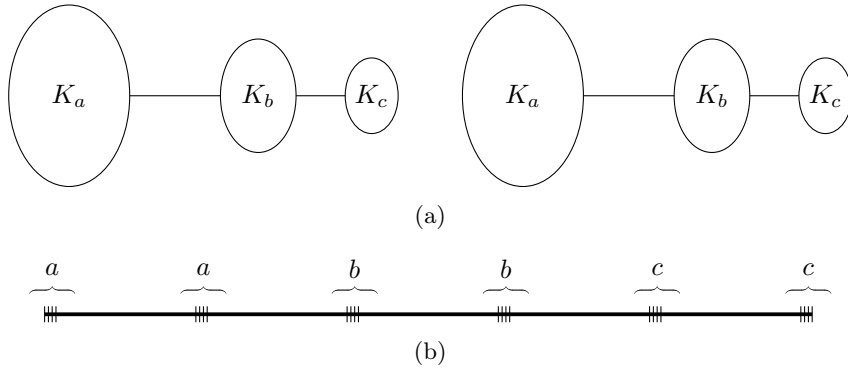
Figure 12: The instance proving Proposition 5.25.
