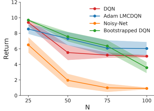
Figure 1: A comparison of Adam LMCDQN and other baselines in N -chain with different chain lengths N . All results are averaged over 20 runs and the shaded areas represent standard errors. As N increases, the exploration hardness increases.
