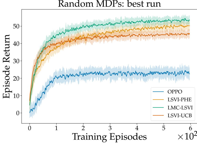
Figure 4: Comparison of LMC-LSVI, OPPO (Cai et al., 2020), LSVI-UCB (Jin et al., 2020) and LSVI-PHE (Ishfaq et al., 2021) in randomly generated non-stationary linearly parameterized MDPs with 10 states, 4 actions, horizon length H = 100 and a sparse transition matrix.
