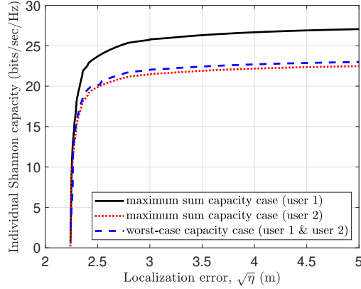
(b) Individual communication capacities vs. target localization error
