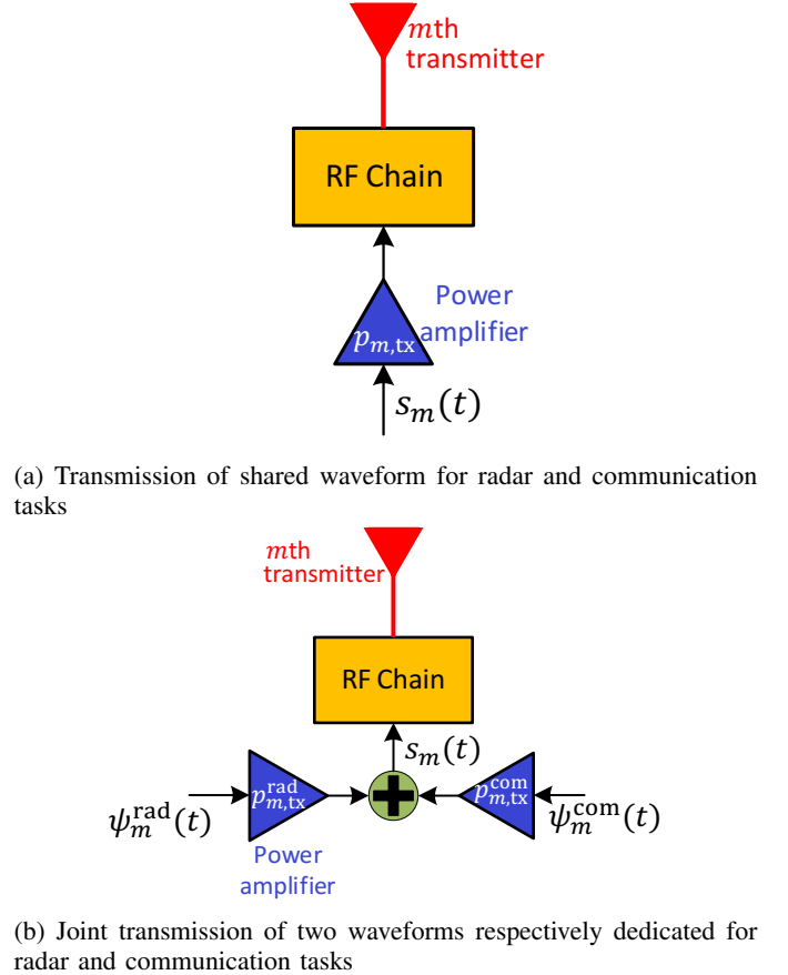
Fig. 3: Transmission strategy at m th transmit antenna ( m = 1, \dots, M ) for distributed MIMO JRC system using shared and dedicated waveforms.
