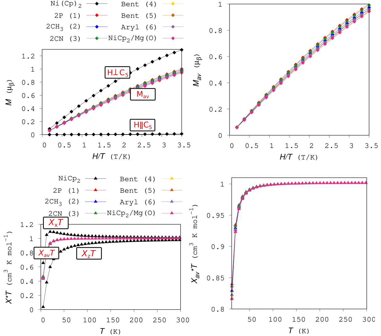
FIG. 7: Calculated field-dependent magnetizations (top) of (i) \text{NiCp}_2 , (ii) six ring-substituted \text{NiCp}_2 compounds, and (iii) \text{NiCp}_2/\text{Mg}_{25}\text{O}_{25} adsorption complex ( T = 2 K). Magnetization is in Bohr magneton ( \mu_B ) units. Calculated \chi_{zm}T , \chi_{xm}T ( \chi_{ym}T ), and \chi_{av}T (bottom) in the temperature range from 5 to 300 K and under an applied field of 1 T. “av” stands for isotropic powder averaging. Properties are obtained by EOM-SF-CCSD/cc-pVTZ calculations, with the exception of complexes 5 and 6 for which we employed EOM-SF-CCSD/cc-pVDZ and of \text{NiCp}_2/\text{Mg}_{25}\text{O}_{25} for which we used SF-PBE0/cc-pVDZ.
