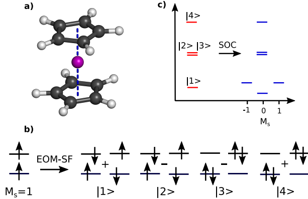
FIG. 1: a) Structures of the nickelocene with staggered rings (coordinates are from Ref. [65]). The bond of the metal with the Cp centroid is shown with dash lines. Color code: Ni — purple, C — gray, and H — white. b) Electronic configurations of the high-spin M_S = 1 triplet reference and the low-spin target states: M_S = 0 triplet ( |1\rangle ) and singlets ( |2\rangle , |3\rangle , and |4\rangle ). State energies and character are obtained from EOM-SF-CCSD calculations. The two closed-shell configurations in states |3\rangle and |4\rangle have equal weights. c) Four lowest electronic states and spin-orbit splitting of the S = 1 ground state. Spin-orbit splitting is computed via a two-step state-interaction scheme.
