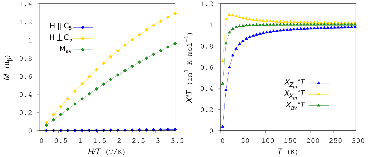
FIG. 5: Calculated field-dependent magnetizations (on the left) of NiCp 2 at low temperature ( T = 2 K). Magnetization is in Bohr magneton ( \mu_B ) units. Calculated \chi_{Z_m} T , \chi_{X_m} T ( \chi_{Y_m} T ), and \chi_{av} T (on the right) of NiCp 2 in the temperature range from 5 to 300 K and under an applied field of 1 T. “av” stands for isotropic powder averaging.
