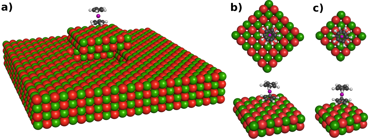
FIG. 3: a) The embedded cluster setup used for structure optimization: the all-electron QM region ( \text{NiCp}_2/\text{Mg}_{49}\text{O}_{49} ) is treated with PBE0/6-31G*, while the outermost region contains point charges. The QM region is shown as lifted for clarity. Here, \text{NiCp}_2 is on-top of \text{Mg}^{2+} adsorption site. b) Top and side views of the embedded \text{NiCp}_2/\text{Mg}_{49}\text{O}_{49} PBE0 region. c) Top and side views of a smaller cut-out ( \text{NiCp}_2/\text{Mg}_{25}\text{O}_{25} ) used for the SF-TDDFT calculations. Color code: Ni — purple, Mg — green, O — red, C — gray, and H — white.
