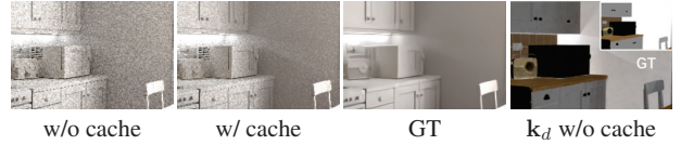
Figure 5: Diffuse radiance cache from L' helps reduce variance and error for shading estimation (2nd image). Without it, sampling the tiny emitters below the cabinet will be difficult (1st image), which leads to incorrect shading and albedo (4th image).
