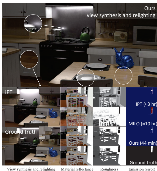
Figure 1: Ours vs standard IPT. IPT [1] takes a piecewise constant parameterization of material to reduce Monte Carlo variance and ambiguity for inverse rendering, losing fine spatial details as a result. Directly extending it to complex material representation (e.g. MILO [45]) shows very slow convergence. In contrast, we propose Factorized Inverse Path Tracing (FIPT) to get rid of variance and reduce ambiguities, yielding efficient and high quality BRDF and emission (4th row), appealing relighting (1st row), and object insertion (the bunny on the table). The presented scene is synthetic with the inset showing the input (lower-left sub-figure). We further showcase results on real scenes in Fig. 10 and 11.
