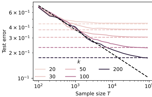
Figure 11: Model Collapse for Hutter++. Empirical confirmation of Theorem 4.2. Here p(j | i) is as in equation 12, with \beta = 7/5 . The horizontal broken lines correspond to k^{-\beta c} for different values of k , where c := \min(1 - 1/\beta, 1/2) . The diagonal broken line corresponds to T^{-c} (classical error rate without cut-off).
