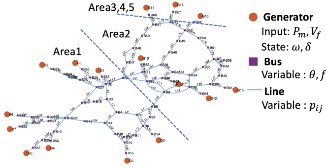
Fig. 1. Diagram of the 68-bus system with 16 generators.
