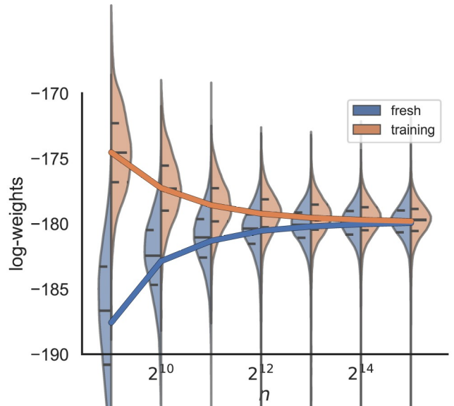
Figure 2: Distribution of log-weights as a function of optimization sample size n (mushrooms dataset). The violin plot shows the distributions, with overlaid lines indicating means for both fresh and training samples. These means provide estimations for the ELBO and training objective.
