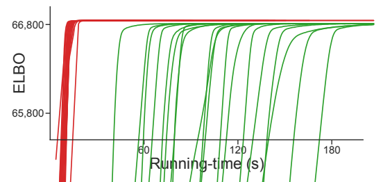
Figure 4: Stochastic volatility model optimized using a diagonal-covariance Gaussian distribution, showing the ELBO achieved by SAA for VI and Adam as a function of time. For Adam, we show the traces corresponding to the best step size of the three used.
