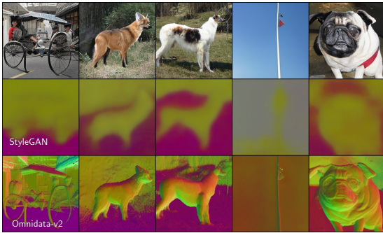
Figure 12: This figure shows the failure in generation of surface normal directions using StyleGAN-XL on ImageNet with 10,000 unique generated images. The images in the middle row resemble the surface normals in the bottom row but miss details that [28] predicted. The differences in architecture between StyleGAN-XL and the more appropriate StyleGAN-2 make it difficult to leverage this model. Either an alternate strategy is required or the latent space in this model is not easy to manipulate.
