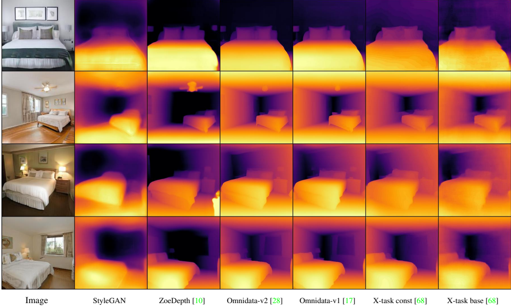
Figure 4: Depth estimation. While fine details may not be as clearly estimated as top methods like ZoeDepth, the overall structure produced by StyleGAN is consistent in quality with recent models.
