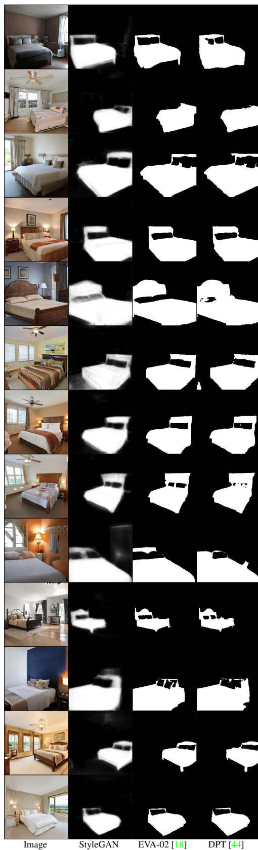
Figure 19: Bed segmentation comparison.
