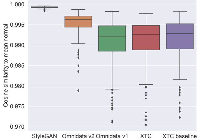
Figure 11: Quantitative evaluation of normal variations following relighting. Normals are calculated under 16 distinct lighting conditions from [11] for 214 test scenes for each normal prediction methods. The inner product between normals under each condition and the overall mean is computed. Ideally, this should be 1, indicating normals’ consistency. The boxplots illustrate these values, with regression methods showing an average change of 8 degrees, with outliers up to 14 degrees. High similarity scores for StyleGAN indicate its normals’ robustness to lighting changes.
