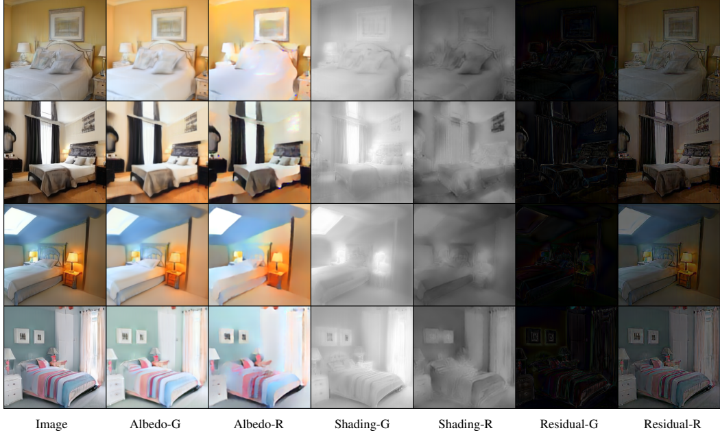
Figure 5: Albedo-Shading Recovery with StyleGAN . We denote results from StyleGAN as -G and from a SOTA regression model [20] as -R. Absolute value of image residuals ( \mathcal{I} - \mathcal{A} * \mathcal{S} ) appears in the last two columns. While our searches for albedo and shading directions were independent, StyleGAN appears to “know” these two intrinsics should multiply to yield the image.
