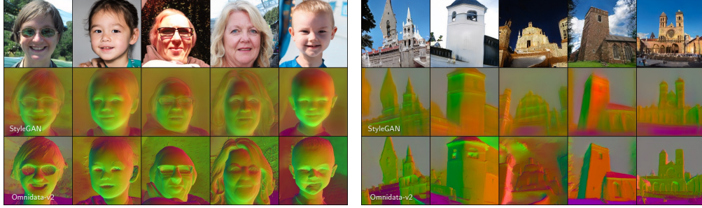
Figure 7: Examples of StyleGAN-generated normals for a StyleGAN model that was trained on the FFHQ dataset (left) and LSUN church (right). Top rows show randomly generated images, middle rows display StyleGAN-generated normals with fixed offset to w^+ codes of top rows and last rows provide Omnidata-v2 Surface Normals for comparison.
