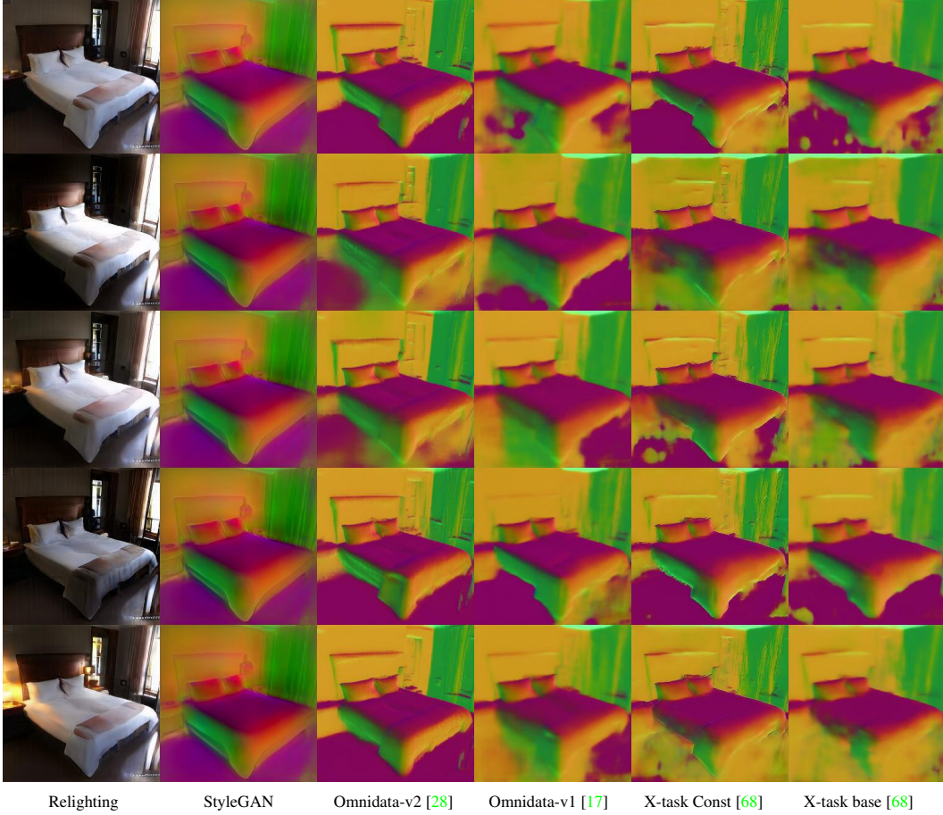
Figure 10: Robustness against lighting changes. Normals should be invariant to lighting changes, yet surprisingly, the top-performing regression methods, even those trained with labeled data, with lighting augmentations and 3D corruptions [28], demonstrate sensitivity to lighting alterations. Intriguingly, StyleGAN-generated normals prove to be robust against lighting alterations.
