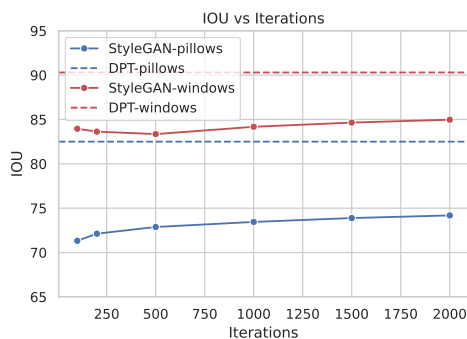
Figure 13: Segmentation Quality vs. Labeled Dataset Size: The graph illustrates how segmentation quality for ‘pillows’ and ‘windows’ classes improves with increasing labeled images, plateauing around 2,000 images. Note that all images are seen only once. While the potential exists for further refinement, the core insight is StyleGAN’s inherent capability to generate these segmentations without explicit training.
