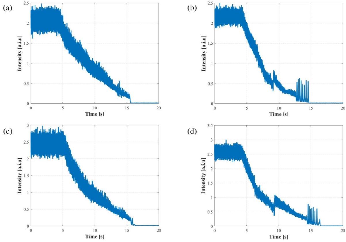
Figure 3. Global chemiluminescence of \text{CH}^* showing heat release rates. Peaks in these graphs demonstrate change in flame shape and extinction/reignition when approaching blowoff: (a) 35 m/s, S = 1.43 ; (b) 35 m/s, S = 0.95 ; (c) 40 m/s, S = 1.43 ; (d) 40 m/s, S = 0.95 .
