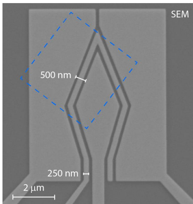
Extended Data Fig. 1: SEM image of the Cr/PdAu bottom gates with the stripe gate width and outer gate widths identified. The blue dashed square indicates the approximate location for the PL diffusion measurements.
