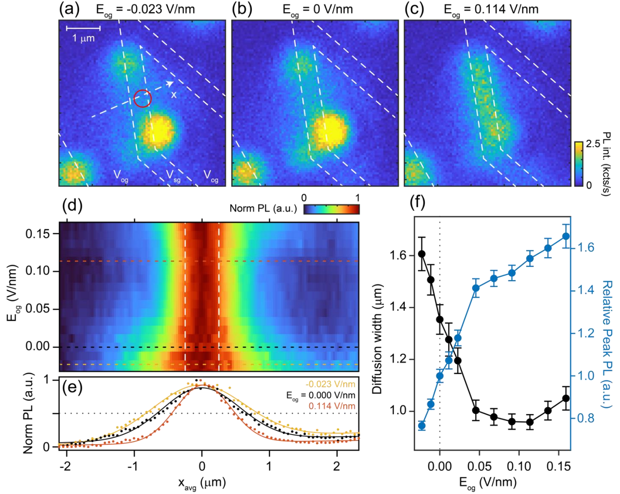
Fig. 2 Controlling the diffusion behavior (a)-(c) Spatial mapping of the diffused IE PL emission at E_{og} = -0.023, 0 , and 0.114 V/nm. The outer gate and the stripe gate areas are labeled V_{og} and V_{sg} , respectively. White dashed arrow indicates positive x direction. Red circle is the excitation position. Bright spots that naturally occur on the sample are reduced with the trapping potential. (d) Normalized PL along the x direction, averaged over the uniform y -cut trap region, as a function of E_{og} . The dotted lines correspond to the E_{og} line cuts in (e). The white dashed lines indicate the expected trap width of \sim 500\text{nm} . (e) Line cuts (scatter) and Gaussian fittings (lines) at E_{og} = -0.023, 0 , and 0.114 V/nm showing narrowing (broadening) of the diffusion width when forming a trap (anti-trap). (f) Extracted diffusion width and relative peak intensity ( PL_{\text{peak}}(E_{og})/PL_{\text{peak}}(E_{og} = 0) ) as a function of E_{og} . We observe the trap saturates near E_{og} \approx 0.04 V/nm.
