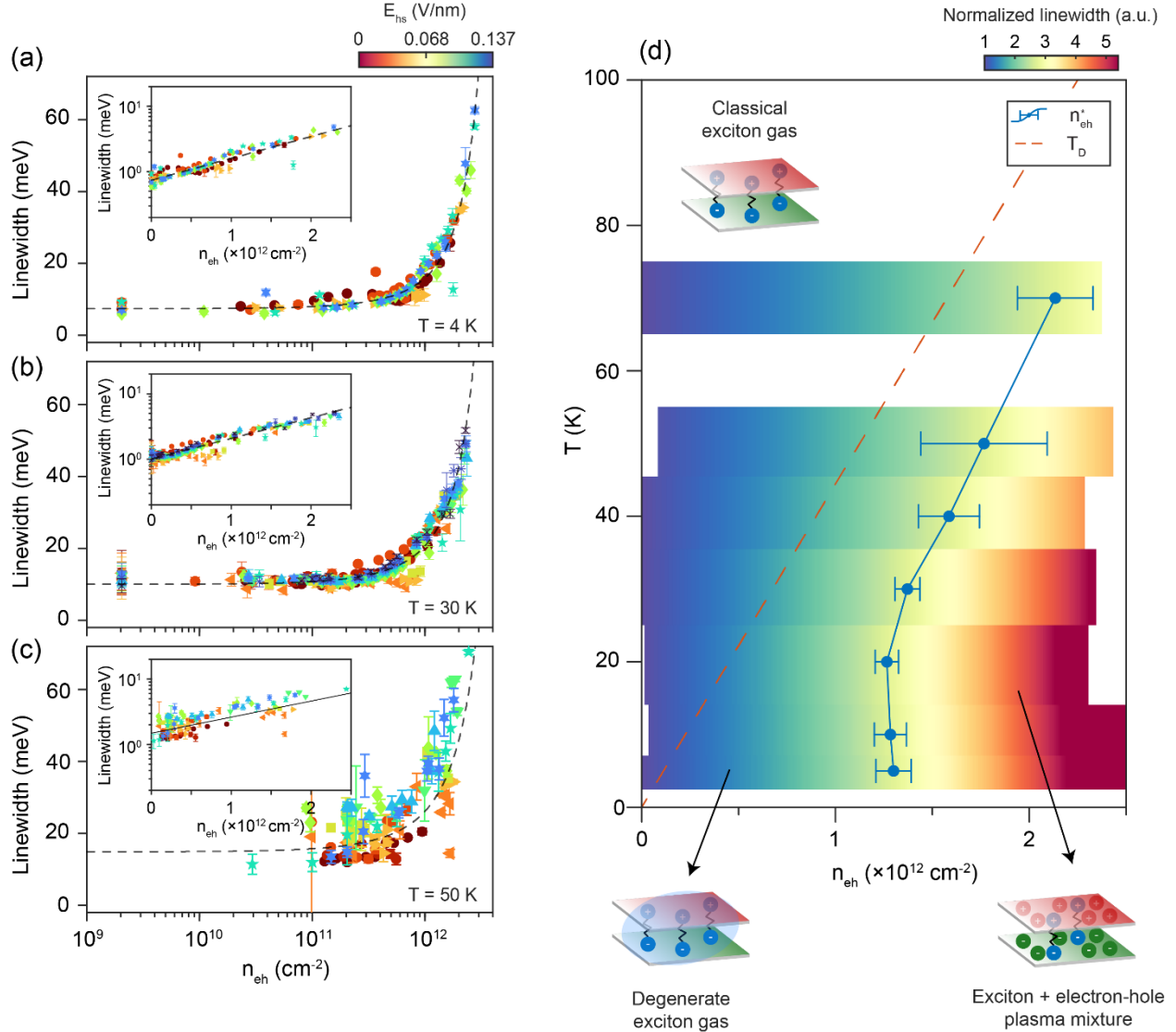
Fig. 4 Interlayer exciton phase diagram (a) Scatter plot of linewidth vs. electron-hole density for various trap depths at T = 4 \text{ K} . The error bars indicate the uncertainty of the fittings. The black dashed line shows the exponential fit giving a universal critical density n_{eh}^*(4\text{K}) = 1.30(\pm 0.09) \times 10^{12} \text{ cm}^{-2} . Inset: Same data but where linewidth is on a log scale and density on linear scaling, showing the exponential fit is shown as a linear curve. (b-c) Same as (a) but at 30 \text{ K} with n_{eh}^*(30\text{K}) = 1.37(\pm 0.06) \times 10^{12} \text{ cm}^{-2} and 50 \text{ K} with n_{eh}^*(50\text{K}) = 1.77(\pm 0.32) \times 10^{12} \text{ cm}^{-2} , respectively. (d) Plot of the fitted normalized linewidth over the collected data range as a function of pair density and measured temperature. The blue data shows the extracted n_{eh}^*(T) at different temperatures with the error bars showing the uncertainty of the fits. The red dashed line is the degeneracy temperature, T_D as a function of exciton density per flavor.
