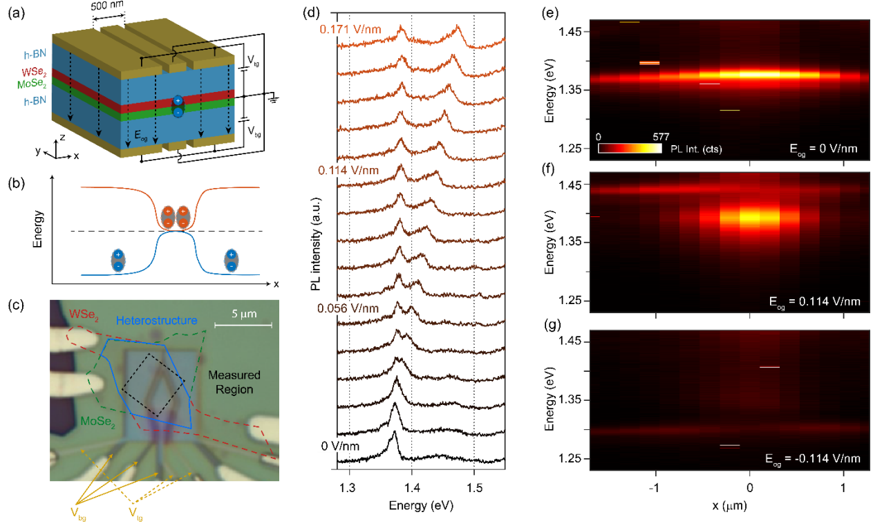
Fig. 1 Modulating the interlayer exciton energy with electric fields (a) Device schematic showing the stripe gate and large outer gates on either side. V_{tg} and V_{bg} are applied to create electric fields in the outer gate ( E_{og} ) regions while the stripe gates are grounded. (b) IE energy schematic as a function of x -position perpendicular to the stripe gate. The red (black dashed) curves represent the electric field profile felt by the IEs with (without) E_{og} in a trapping configuration. The blue curve represents the anti-trap regime. (c) Optical image of the device. Red and green dashed lines outline the WSe 2 and MoSe 2 regions, respectively. Blue line outlines the heterostructure region. Gold arrows identify the relevant top gate and bottom gate structures. The black dashed square indicates the approximate region for the PL diffusion measurements. (d) IE spectra as a function of E_{og} . The linearly shifting peak at higher energy is from the outer gate region while the lower energy peak is from within the stripe gate region. (e)-(g) Scanning PL spectroscopy, where the laser excites at x = 0 \mu\text{m} and the spectra is collected across the stripe gate at E_{og} = 0 and \pm 0.114 \text{ V/nm} , showing spatially modulated IE energy.
