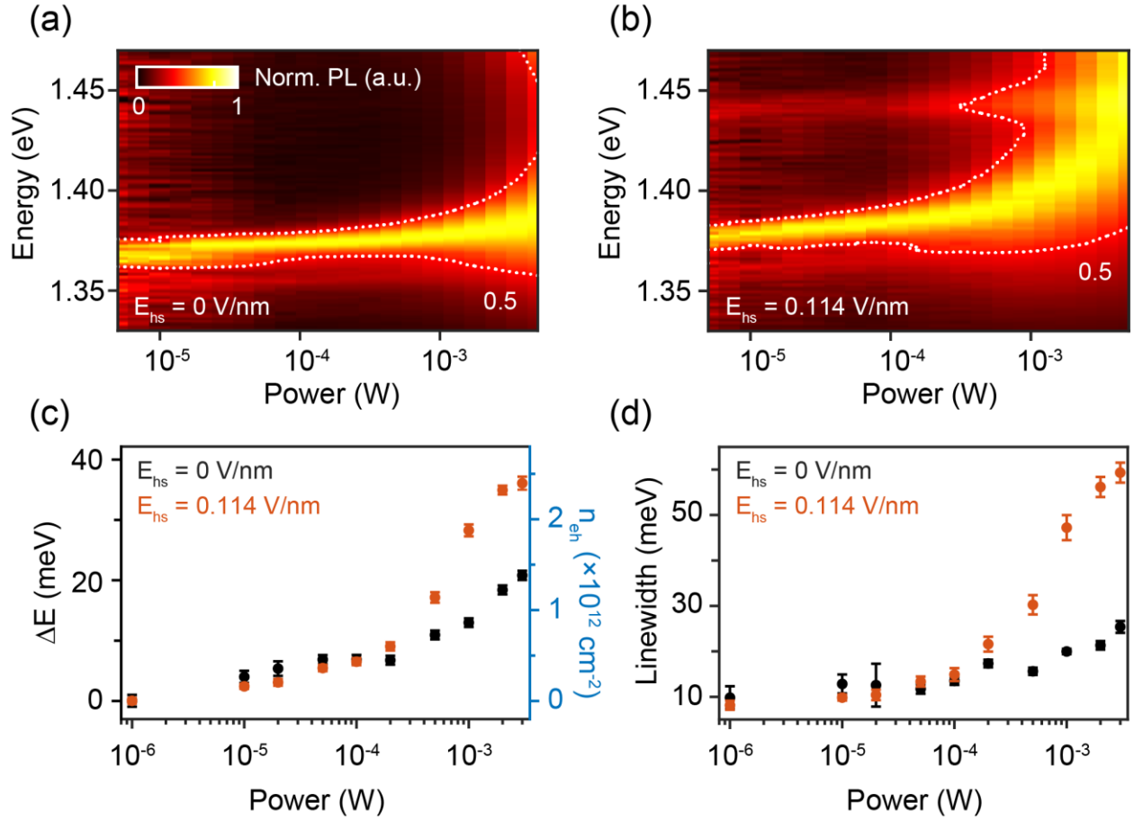
Fig. 3 Tuning the interlayer exciton density (a) Normalized power dependent PL emission from the stripe gate region at E_{og} = 0 V/nm, when the excitation laser is slightly outside the region. The dotted white line shows a contour of 0.5 for the intensity of the trapped IEs. (b) Same as (a) for E_{og} = 0.114 V/nm. (c) The blueshift energy, \Delta E , for E_{og} = 0 and 0.114 V/nm as a function of power. Right axis (blue) shows the corresponding calculated electron-hole pair density, n_{eh} . (d) Fitted trapped PL linewidth for E_{og} = 0 and 0.114 V/nm as a function of power. The error bars in (c) and (d) are from the fitting of the spectral peaks.
