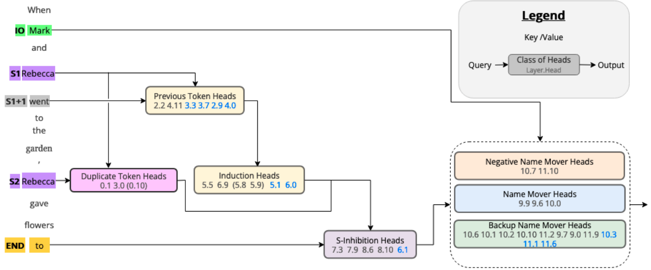
Figure 17. The circuit discovered post-reversal after corruption on Name Moving Augmentation, the new components are marked in blue.
