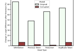
Figure 9. Subject Duplication: Change in Logit Difference after ablating groups of heads.
