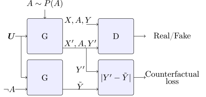
Figure 2: Counterfactual Fairness
