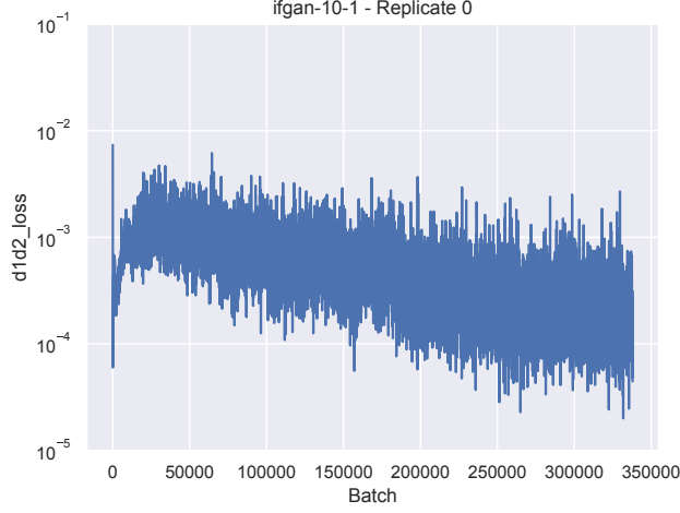
Figure 7: \lambda = 10^{-1}
