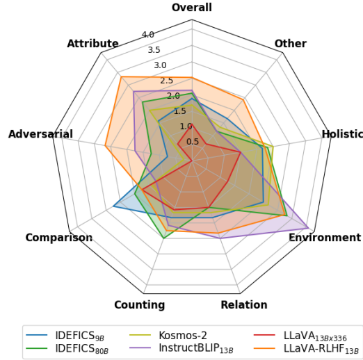
Figure 2: Detailed performance of different models on the eight categories in MMHAL-BENCH, where “Overall” indicates the averaged performance across all categories. The questions are collected by adversarially filtering on the original LLaVA 13Bx336 model.
