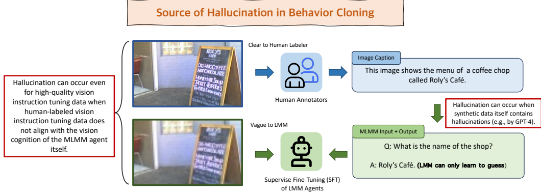
Figure 3: Two sources of hallucination in Supervised Fine-Tuning (SFT): GPT-4 synthesized data contains hallucinations; Instruction data labelers have no insights about what LMMs know or see, which essentially teaches them to speculate on uncertain content (i.e. hallucinate).
