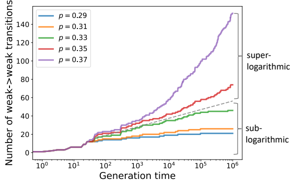
Figure 5. Growth of weak to weak transition
