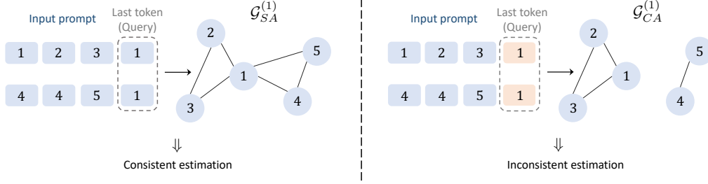
Figure 3. Illustration of co-occurrence graphs for the self-attention ( Left ) and cross-attention ( Right ) models. We fit the same input examples where the only difference is the use of self- vs cross-attention (which includes vs excludes the query token ‘1’ from the list of key tokens). Following Theorem 3.4, in the cross-attention setting, where the token ‘1’ is not contained in the prompt, the co-occurrence graph becomes disconnected, resulting in inconsistent estimation. In contrast, the estimation is consistent for the self-attention model since both inputs share the same query token within their key tokens.
