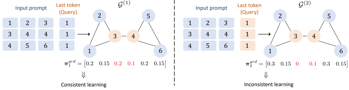
Figure 6. Illustration of the Co-occurrence Graphs for the Cross-attention Models with Possible Zero Transition Probability in \mathbf{P}^{\text{GT}} . In this figure, we draw the co-occurrence graphs of the input prompt distribution whose support consists of three elements under the cross-attention model. In the left figure, the first column of the transition matrix \mathbf{P}^{\text{GT}} does not include any zero transition whereas, in the right figure, the first column of the transition matrix \mathbf{P}^{\text{GT}} includes zero transition. For the left figure, the co-occurrence graph \mathcal{G}^{(1)} is connected with respect to \mathbf{P}^{\text{GT}} . However, in the right figure, the co-occurrence graph \mathcal{G}^{(1)} is not connected with respect to \mathbf{P}^{\text{GT}} as there is no path between 2nd vertex and the 5th vertex using non-zero vertex.
