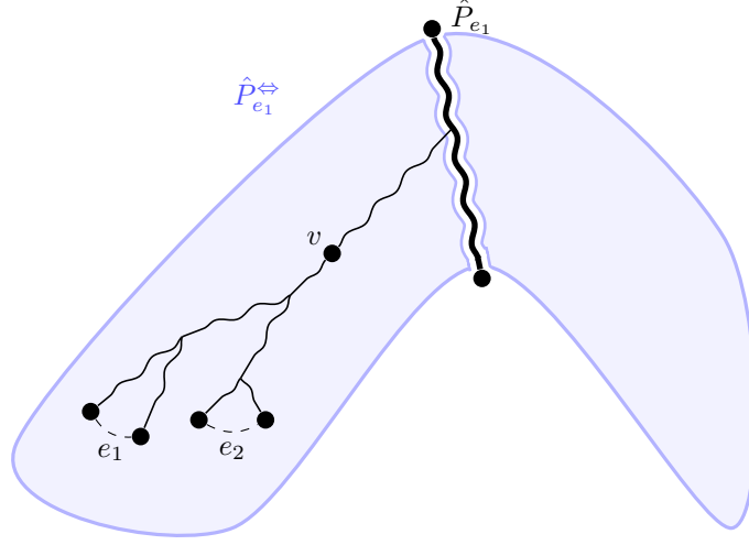
Figure 4: An illustration to Lemma 5.11: if the algorithm arrives at vertex v but has not found any lower vertex for e_1 and e_2 yet, then \hat{P}_{e_1} = \hat{P}_{e_2} .
