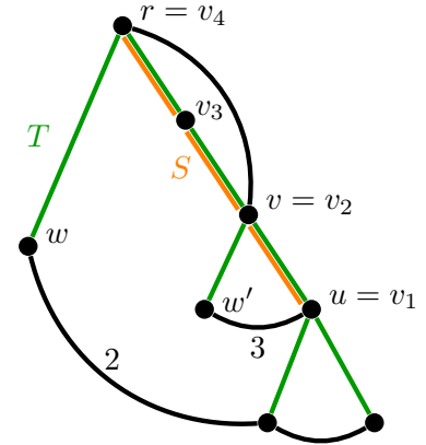
Figure 5: A Missing Case.
