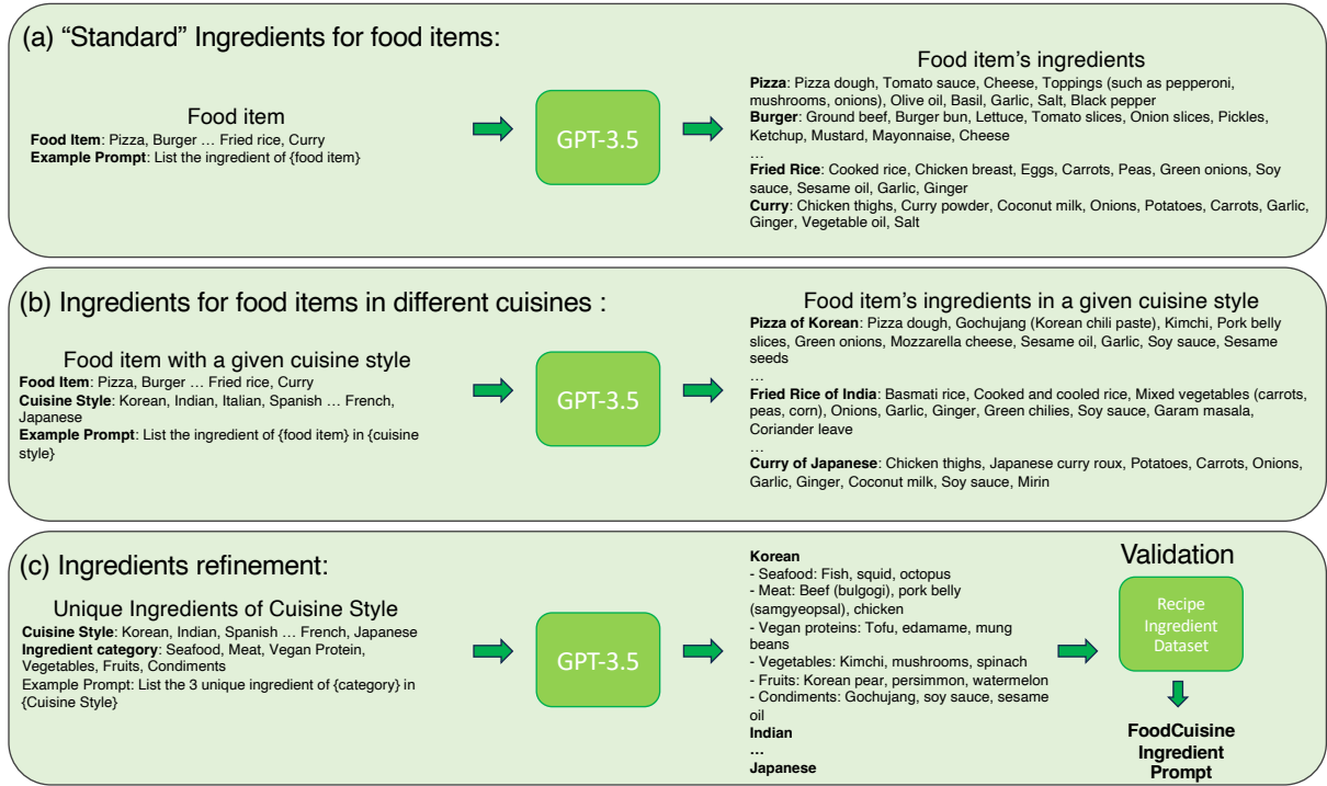
Figure 2. Prompt generation for ingredients of food items in distinct cuisine style: (a) Generating a comprehensive ingredient list of standard culinary preparation. (b) Generating cuisine-specific ingredients list of culinary items. (c) Refining the cuisine-specific ingredients list based on uniqueness
