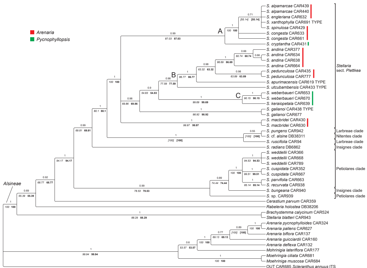
Fig. 4. Bayesian majority rule consensus tree inferred from nuclear ribosomal (ITS) sequence matrix including indels. DNA posterior probabilities are above branches, parsimony jackknife values are below branches left and in italics, and maximum likelihood bootstrap percentages right and in bold. The monophyletic Stellaria sect. Plettkea is deeply nested within the genus Stellaria . Species previously classified within Arenaria and Pycnophyllopsis are annotated with a red or green bar, respectively.
