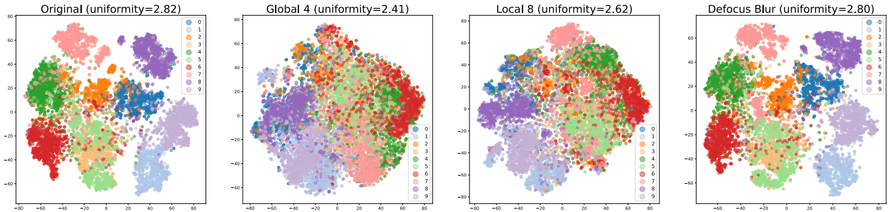
Figure 3: t-SNE visualizations of features from MoCo-v2 Original (1st), Global 4 (2nd), Local 8 (3rd) and Defocus Blur (4th) pre-trained on CIFAR-10. We observe that corrupting spatial inductive bias can effectively undermine a well-clustered feature space.
