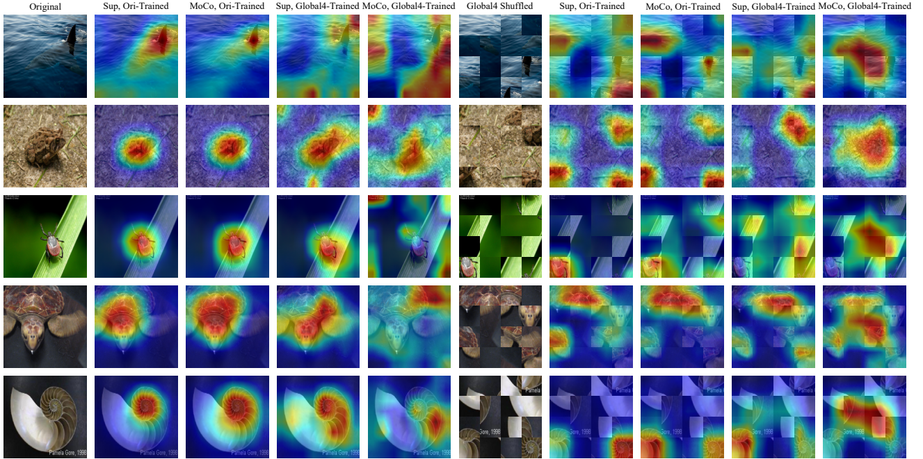
Figure 2: For several ImageNet-100 images, we visualize the Grad-CAM activation maps of 4 models: SL ('Sup') and MoCo-v2 ('MoCo') with ResNet backbone trained on original images, along with SL and MoCo-v2 trained on images corrupted by global patch shuffling. The activation maps of MoCo-v2 trained with corrupted images are mostly different from the reference (SL or MoCo-v2 trained with original ImageNet), and are the most diffused and messy ones.
