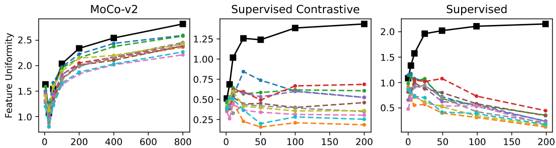
Figure 4: Uniformity of MoCo-v2, supervised contrastive learning, and SL with training epochs on CIFAR-10. Solid black line – uniformity of the overall feature space. Dashed lines – class-wise feature uniformities of the 10 classes. While the overall uniformity of all methods grows, the uniformity of each class of Sup or SupCon is shrinking as training progresses. In the end, the overall uniformity of MoCo is the largest.
