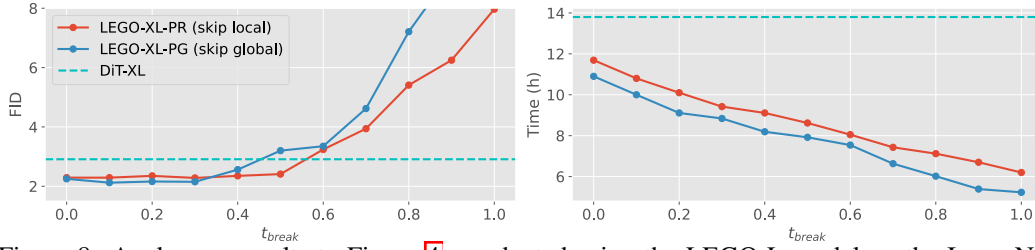
Figure 8: Analogous results to Figure 4, conducted using the LEGO-L model on the ImageNet ( 64 \times 64 ) dataset with classifier-free guidance.
