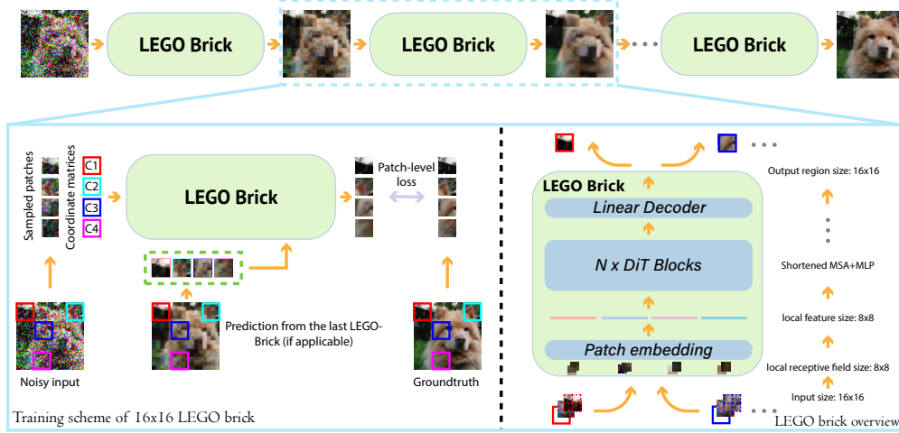
Figure 3: Top Panel: The generation paradigm with LEGO spatial refinement in a single time step. Bottom Panel: An overview of the training scheme ( Left ) and architecture ( Right ) of a LEGO brick, whose input size is 16 \times 16 , local receptive field size is 8 \times 8 , and attention span is 4.
