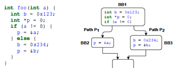
Figure 4: An example illustrating the data-flow analysis in TYGR. (Left) A simple function with two possible paths. (Right) The control-flow graph of the function.
