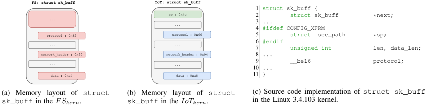
Fig. 1: Example of the misaligned data structure struct sk\_buff . Figures 1a and 1b illustrate the incorrect and correct offsets of the misaligned members of struct sk\_buff (red and blue shapes, respectively). Here the analyst has to enable the configuration option CONFIG_XFRM during FirmSolo’s kernel build process to align the members protocol , network_header , and data at the correct offsets.
