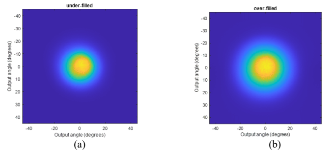
Fig. 2. FFP images at the output of a 15-m SI-POF for the selected launching conditions: (a) UF, (b) OF.
