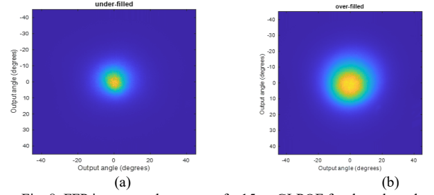
Fig. 8. FFP images at the output of a 15-m GI-POF for the selected launching conditions. (a) UF, (b) OF.
