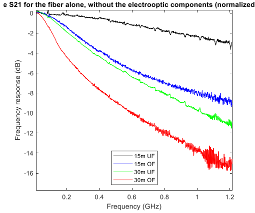
Fig. 7. Magnitude of S21 for 15 meter and 30-meter SI POFs with UF and OF launching conditions.
