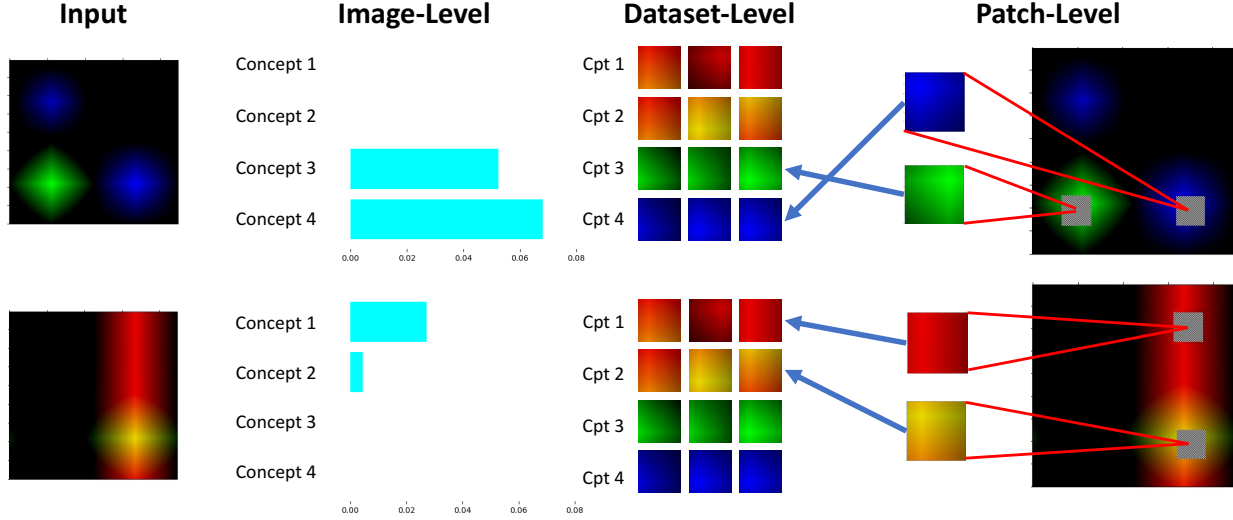
Figure 4. PACE’s three-level conceptual explanations on the Color dataset. Dataset-Level: PACE’s top 4 dataset-level concepts; for each concept k , we plot the top 3 patches with \mathbf{e}_{m,j} closest to \mu_k . Image-Level: Given an input image m , we show PACE’s generated image-level explanation \theta_m for the 4 selected concepts. For example, for the top-left input image, PACE’s generated image-level explanation \theta_m indicates a strong association with Concept 3 (green) and Concept 4 (blue). Patch-Level: Given an input image m , PACE’s \phi_{m,j} identifies the top concepts for the selected patches. For example, for the top-left input image, the blue patch is associated with Concept 4 (containing similar blue patches across the dataset) while the green patch is linked to Concept 3 (containing similar green patches across the dataset).
