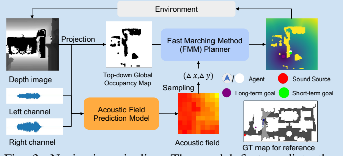
Fig. 3: Navigation pipeline. The model first predicts the acoustic field, samples the peak as the long-term goal, and navigates toward the goal with a path planner.
