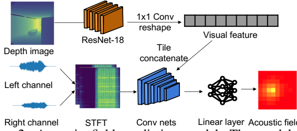
Fig. 2: Acoustic field prediction model. The model extracts audio and visual features, and then tiles, and concatenates both features to predict the acoustic field.
