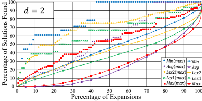
Figure 5: Solutions found vs. percentage of expansions.
