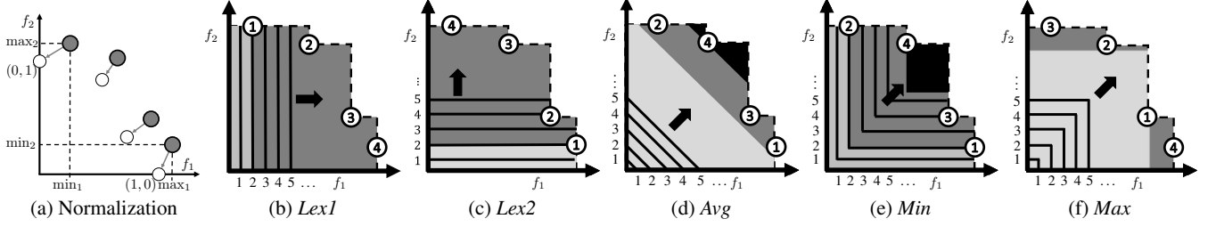
Figure 4: The progress of different ordering functions. The three phases are colored differently.
