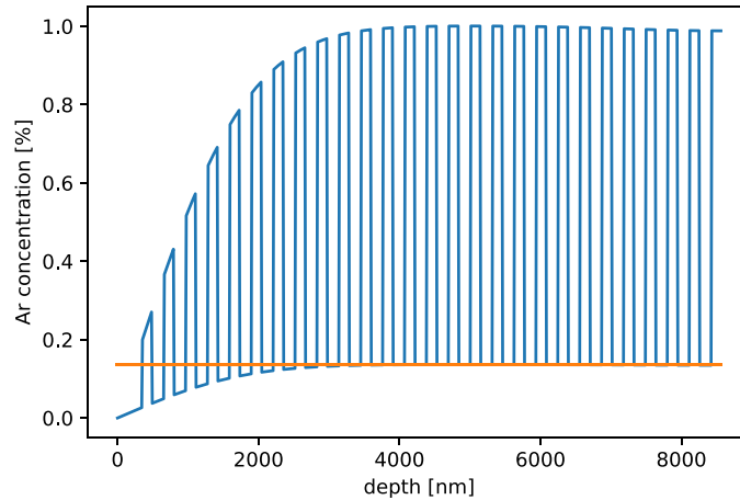
Figure 8. Blue curve: concentration of Ar as a function of depth in a 8.5\ \mu\text{m} stack after a 10 h annealing at 600\ ^\circ\text{C} , according to the transport model. Higher Ar amounts are found in the TGO layers while lower amount corresponds to the Ar content in \text{SiO}_2 layers. Orange line: ratio D_{\text{TGO}}/D_{\text{SiO}_2} = 1/7.3 .
