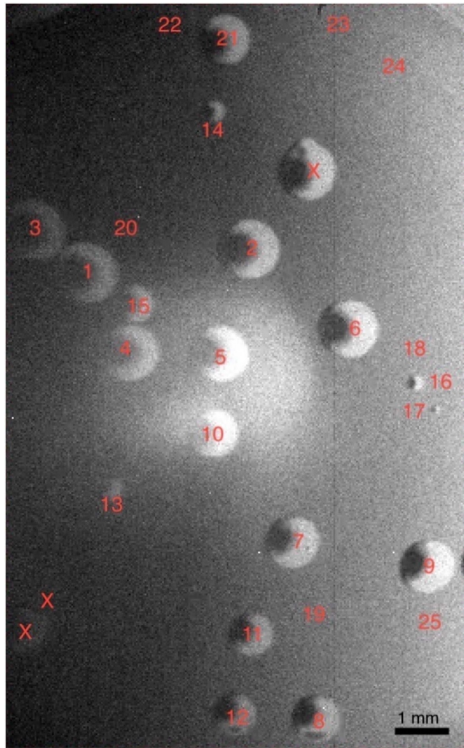
Figure 10. Video frame (at T=522 °C) of blisters growing in the stack deposited on standard-polished fused silica. The 25 tracked blisters are identified by a number (including some that did not yet start to grow at that temperature yet), while a few that were not tracked are marked by an 'X'.
