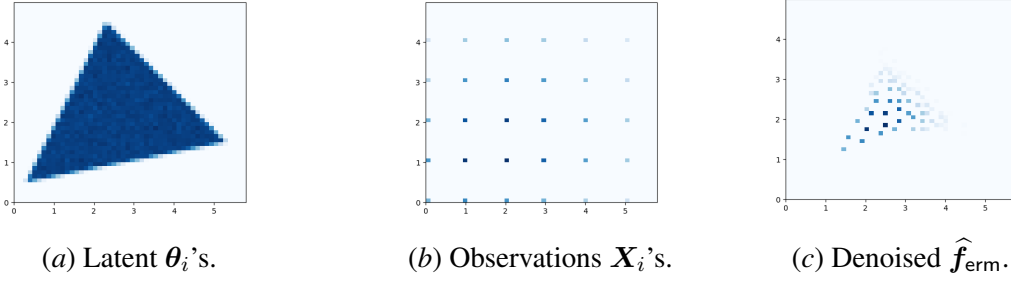
Figure 1: A two-dimensional experiment with n = 10^6 : Left: \theta_i 's are sampled uniformly from a triangle. Middle: the observations X_i 's are drawn independently from \text{Poi}(\theta_i) , with their empirical distribution shown on the grid \mathbb{Z}_+^2 (notice that this is also the MLE estimator for \theta , hence very different from the empirical Bayes solution). Right: the empirical Bayes denoised version obtained by applying \hat{f}_{\text{erm}} in (10) to X_i 's.
