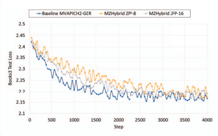
(c) MZHybrid: Books3 test loss
