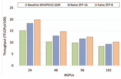
(b) Naive ZFP: TFLOPS per GPU
