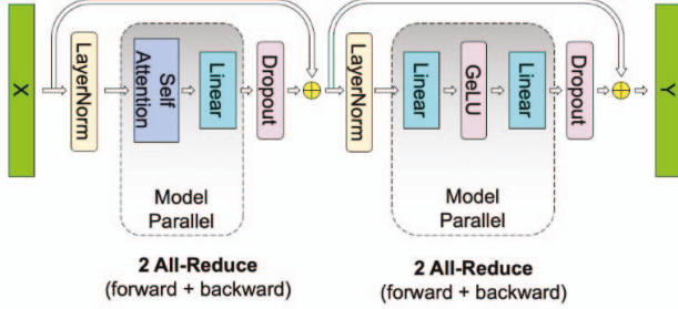
Fig. 3: Megatron-LM: communication primitives involved in a single transformer layer [20].
