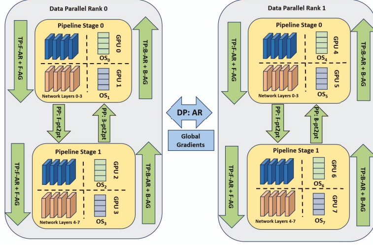
Fig. 2: A base 3D parallelism setting with a total of 8 GPUs. This setting contains two data parallel ranks, two pipeline stages and two tensor parallel degree. Collective operations for each parallelism degree are detailed. Optimizer states are also split across 8 workers. DP : Data Parallelism, PP : Pipeline Parallelism, TP : Tensor Parallelism, OS : optimizer state shards with device index as subscript. AR : All-reduce operations. AG : All-gather operations. F and B prefix indicates forward passes and backward passes respectively.
