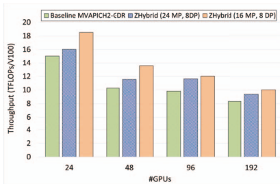
(b) ZHybrid: TFLOPS per GPU
