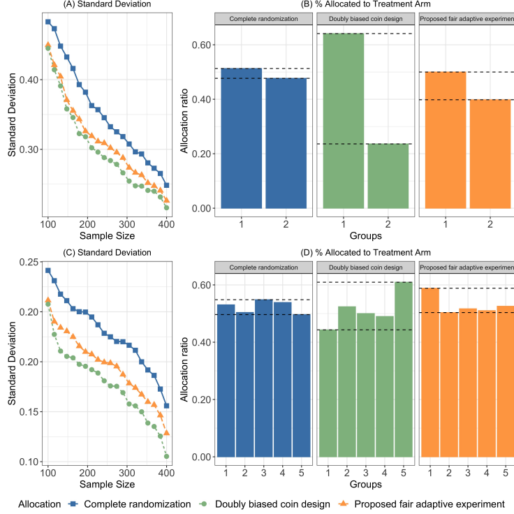
Figure 1: Comparison of the proposed adaptive experiment design strategy, the complete randomization design, and the doubly adaptive biased coin design. (A) and (C) show the standard deviation comparisons. (B) and (D) show the percentage of participants allocated to the treatment arm in each group under different experiment strategies.
