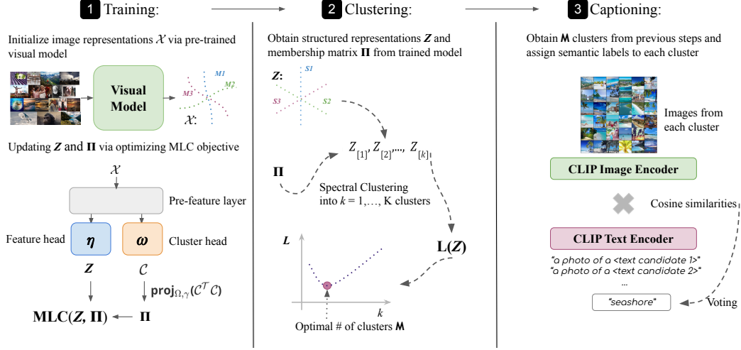
Figure 1: Overall pipeline of CPP. Left: In the training stage, CPP initializes the features \mathcal{Z} and cluster membership \mathbf{\Pi} from a large pre-trained model, and updates \mathcal{Z} and \mathbf{\Pi} by optimizing the (MLC) objective. Middle: Once training is done, CPP selects the optimal number of clusters via the coding length L(\cdot) criteria. Right: CPP assigns semantic captions to each cluster via computing cosine similarities between text candidates and images and voting for the most suitable caption.
