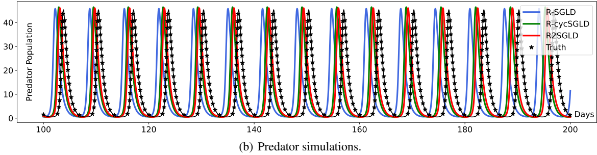
Figure 9. Simulation of the identified Lotka-Volterra system from 100 to 200 days.
