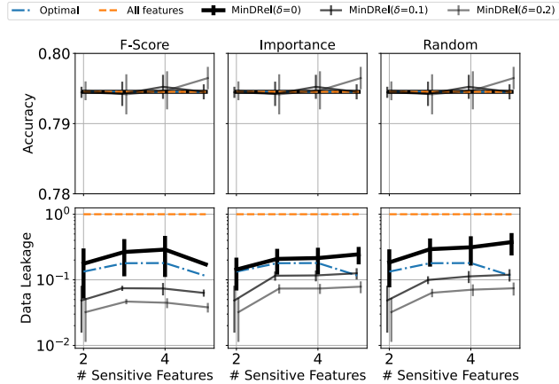
Figure 5: Comparison of F-Score, Importance and Random method for different \delta with two baseline methods: Optimal and All features in term of Accuracy and Data Leakage. The underlying classifier is a logistic regression classifier.
