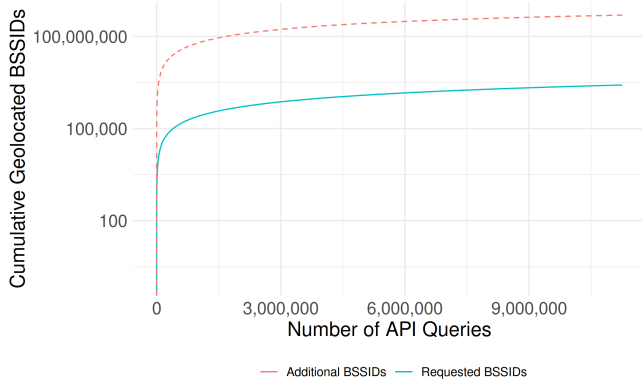
Figure 2: Number of BSSIDs discovered by guessing randomly among IEEE-assigned OUIs and their locally-administered versions versus the additional BSSIDs the Apple Wi-Fi geolocation API returns. Note that the y -axis is log-scale.
