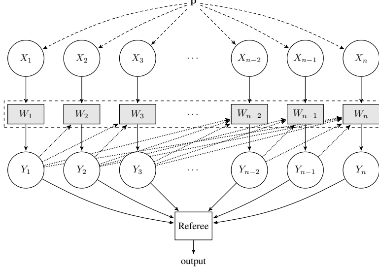
Figure 1: The information-constrained distributed model. In the interactive setting, W_t can depend on the previous messages Y_1, \dots, Y_{t-1} (dotted, upwards arrows).
